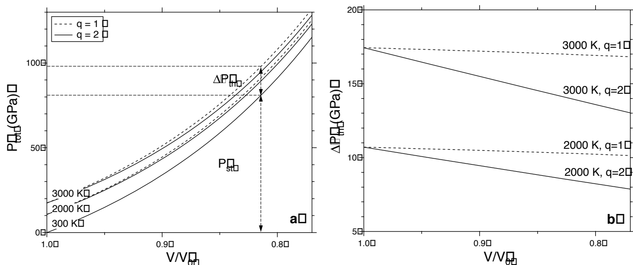
FIGURE 1. The (a) isotherms and (b) thermal pressure calculated using the BMD equation with the thermoelastic parameters of \text{MgSiO}_3 perovskite (Table 1) vs. normalized volume. To illustrate the effect of variations in q , we calculated isotherms for q = 2 (solid lines) and q = 1 (dashed lines).
