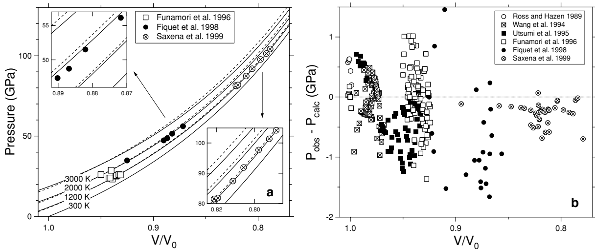
FIGURE 8. Equation of state fit to currently available data sets. (a) Isotherms for 300, 1200, 2000, and 3000 K for fits to LPT (dashed lines) and LPT+FI+SA (solid lines) data sets (see Table 3). Some of the measured data points at 1200 \pm 100 K and 2000 \pm 100 K are plotted for comparison. (b) The difference between the measured pressure and calculated pressure from fitted results for LPT data ( q = 1 ) vs. volume. Estimated errors are smaller than symbol size for both plots.
