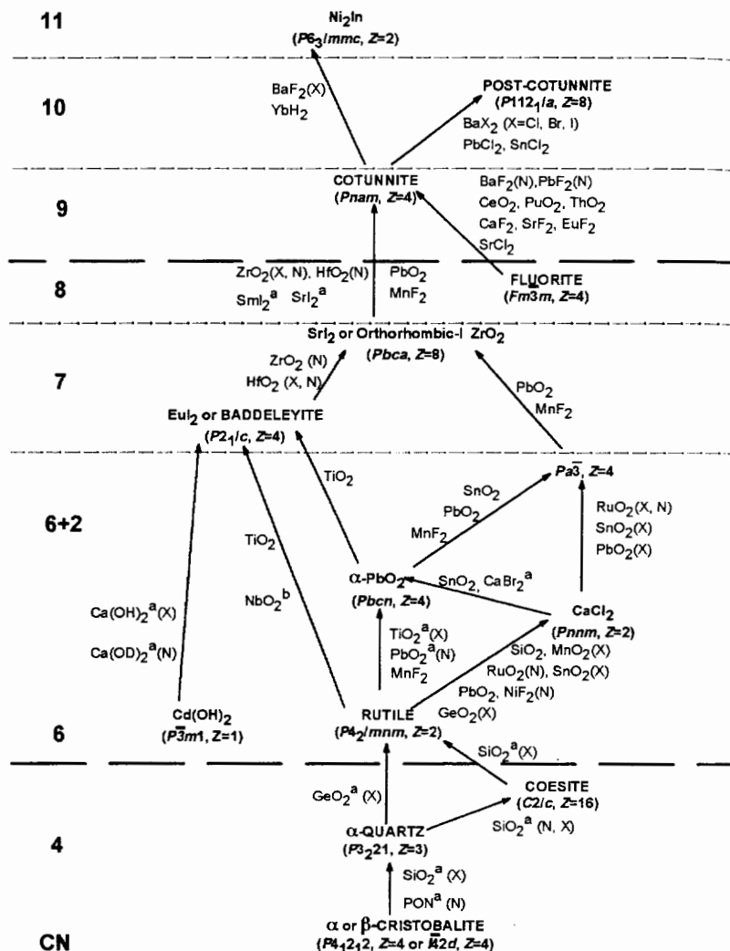
Figure 1: Structure map of the AX_2 compounds as a function of coordination number. Arrows indicate high pressure phase transformations. Examples are given and are labelled X or N where the structure of the high pressure phase has been refined from x-ray or neutron diffraction data, respectively (a: high pressure, high temperature conditions; b: distorted rutile - distorted baddeleyite).
