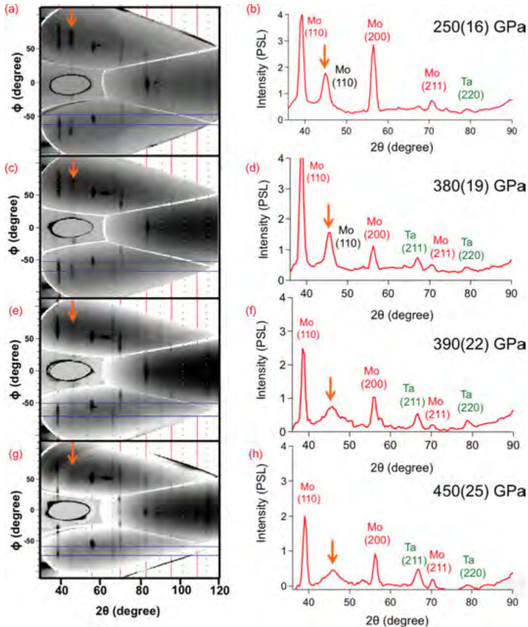
FIG. 4. (Color online) Representative x-ray diffraction data for shock-compressed Mo projected into 2\theta - \phi space [43], where \phi is the azimuthal angle around the incident x-ray direction [panels (a), (c), (e), and (g)]. In these coordinates diffraction peaks are straight lines of constant 2\theta . The vertical solid red lines and dashed green lines show positions of ambient-pressure Mo and Ta peaks, respectively. The orange arrows point to the location of the compressed Mo (110) peak for pressures below 380 GPa and diffuse scattering at higher pressures. The panels on the right [(b), (d), (f), and (h)] show the corresponding background-subtracted one-dimensional x-ray diffraction patterns for the window regions defined by the horizontal blue lines in the corresponding left-hand panel. The diffraction peaks are assigned to uncompressed Mo (red labels), compressed Mo (black labels), and Ta pinhole (green labels). Intensities in the right-hand panels are in photostimulated luminescence (PSL) units.
